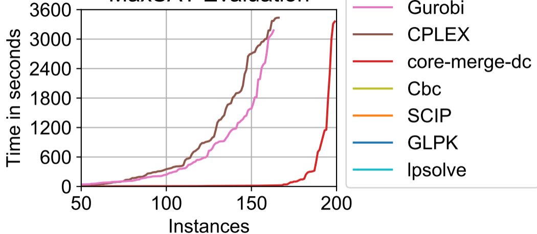
MaxSAT Evaluation
